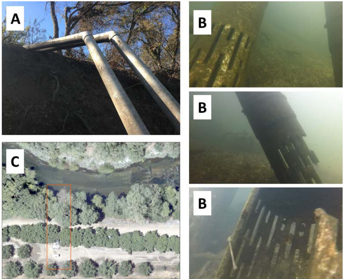
Figure 3. Photographs of Site #2 including; A) the diversion pipes, B) the submerged diversion intakes, C) an aerial view of the site.
