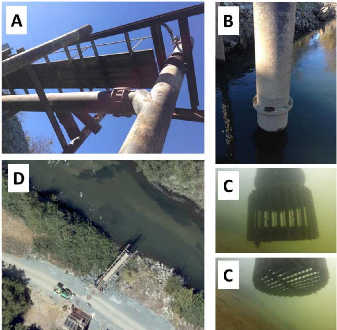
Figure 2. Photographs of Site #1 including; A) the diversion platform, B) the connecting pipe, C) the submerged intake, D) an aerial view of the site.
