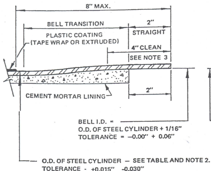
TYPICAL BELL END DETAIL
