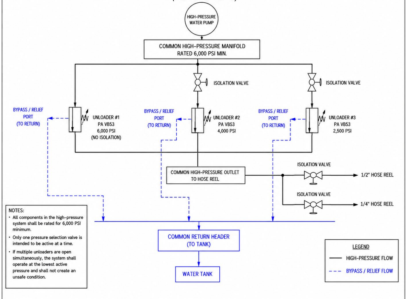
FIGURE 1 – CONCEPTUAL PRESSURE SELECTION MANIFOLD (CONCEPTUAL ONLY)
