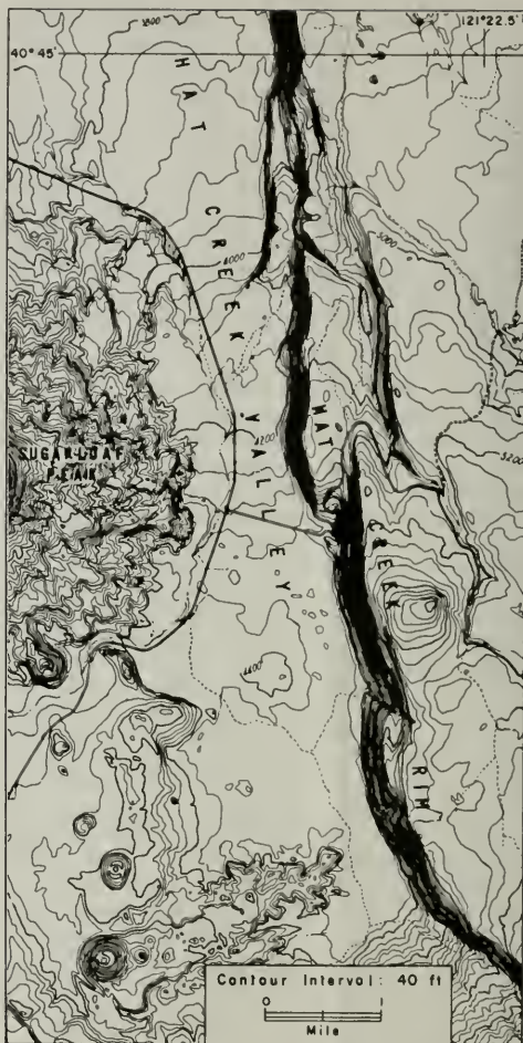
Figure 4. Topographic map of part of the Prospect Peak quadrangle, showing the Hat Creek fault scarp along the eastern edge of Hat Creek Valley. The plateau on the right of the scarp is capped with Burney Basalt. Sugarloaf Peak, on the left, is a late Pleistocene cone built largely of andesite block lava flows. The valley is flooded by the Hat Creek lava flow, which only a few thousand years ago poured out of inconspicuous vents located 2 miles north of the south boundary and 1 mile east of the west boundary of the figure.
