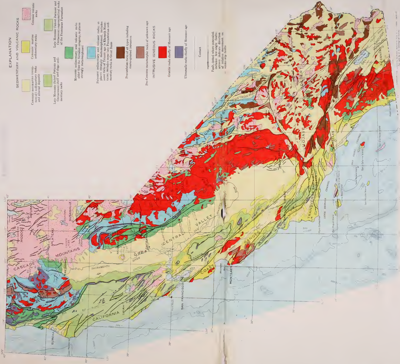
GEOLOGIC MAP OF CALIFORNIA COMPILED BY U.S. GEOLOGICAL SURVEY AND CALIFORNIA DIVISION OF MINES AND GEOLOGY
