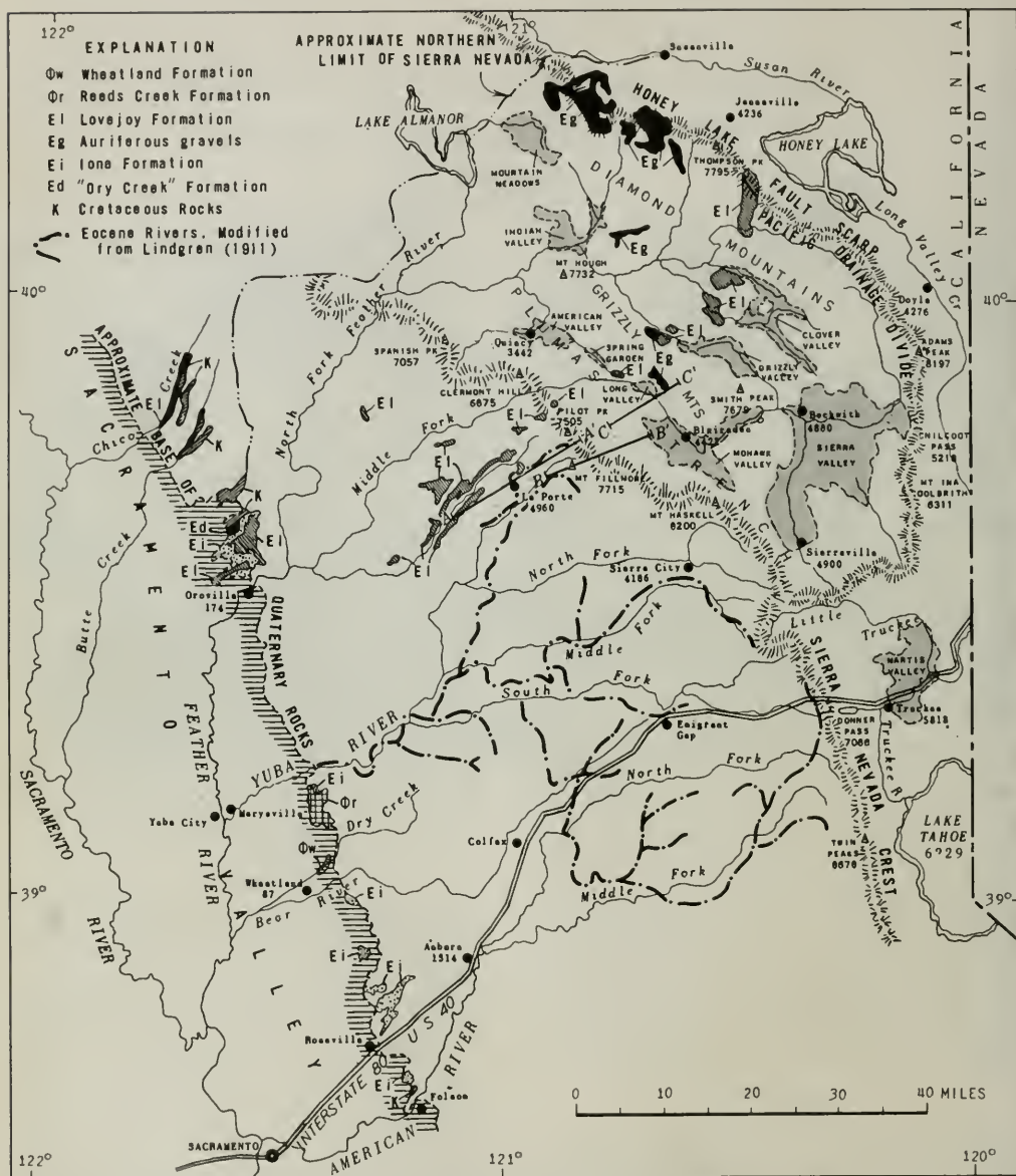
Figure 1. Map of the northern Sierra Nevada, showing geographic features, distribution of Cretaceous and older Tertiary rocks, and the Eocene River system. Lines A-A', B-B', and C-C' show positions of cross sections shown on figure 3.
