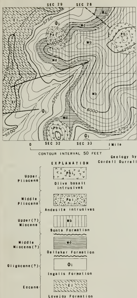
Figure 4. Geologic map of a small portion of the Bloirsdon quadrangle, Plumas County, California, showing reversal of fault movement.
