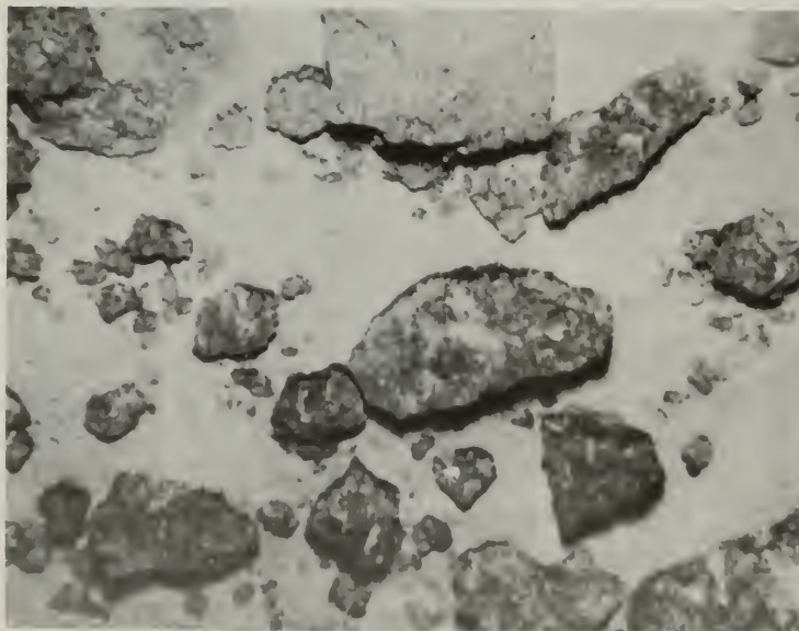
Photo 5. Manganese nodules on the ocean floor at N. 26°, W. 135°, in 4,330 m. of water between California and Hawaii. The largest slablike nodule is about 23 cm in diameter. Many of the blocklike nodules in this photo may be only manganese dioxide encrusted blocks of pumice. Photo by Carl Shippek, U.S. Naval Electronics Laboratory, San Diego, California.
