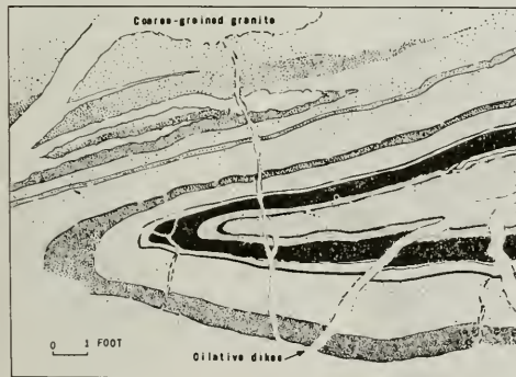
Figure 5. Recumbent folds and granitic dikes in layered gneiss consisting of various proportions of hornblende, plagioclase, and clinopyroxene. Sketched from exposure in vertical roadcut near Escandido Camp, 5 miles west of Junipero Serra Peak.
