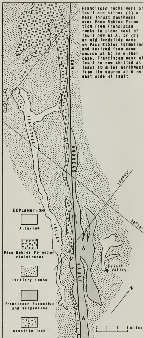
Figure 2. Evidence of late Quaternary right-lateral offset on San Andreas fault in the Peachtree Valley area.
