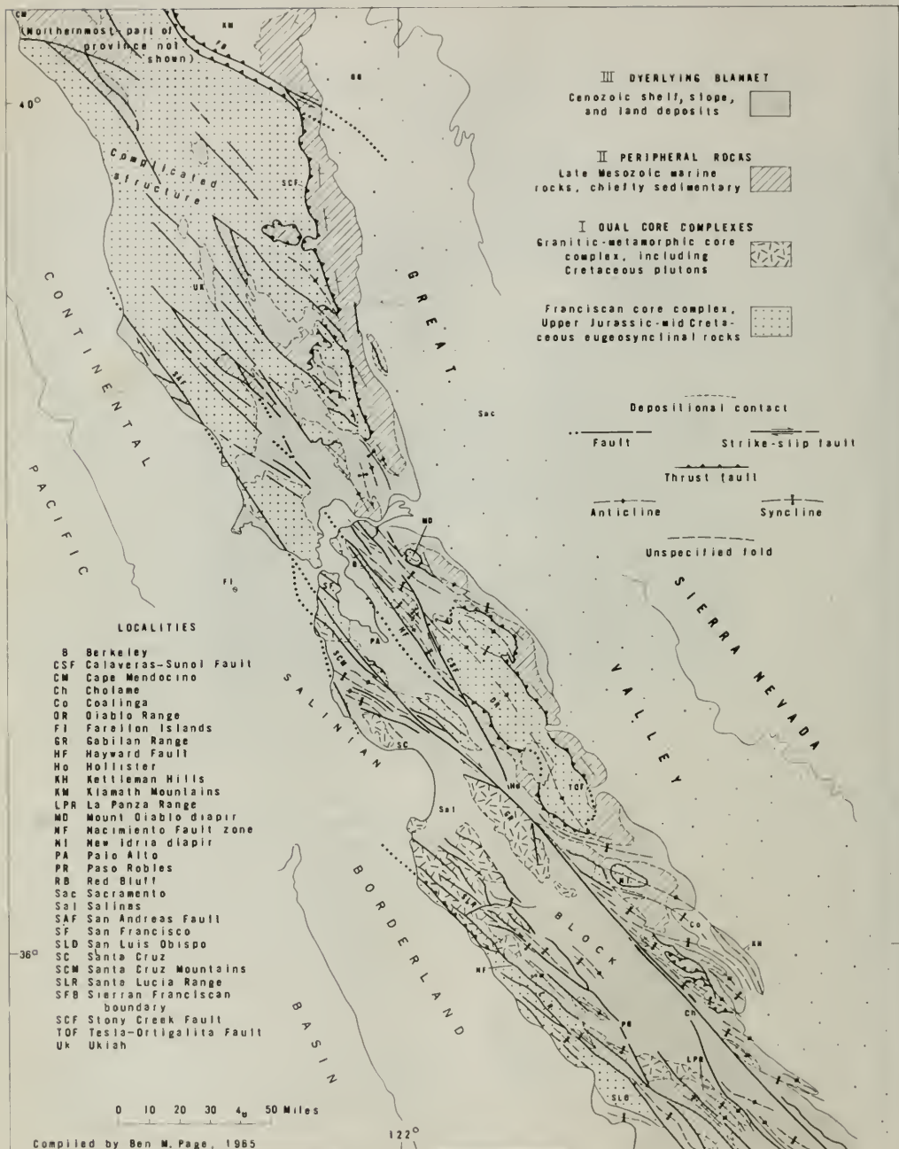
Figure 1. Tectonic map of the California Coast Ranges.
