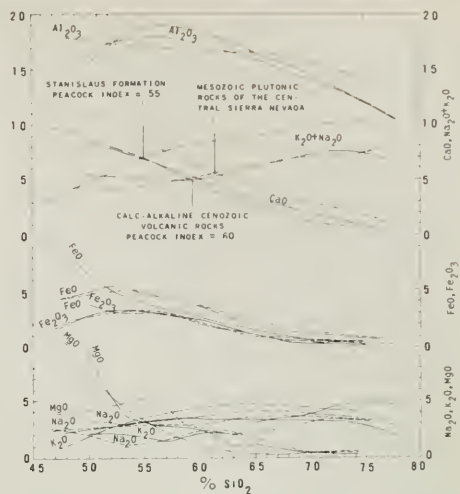
Figure 5. Silica variation diagram for Cenozoic volcanic rocks of the alkalic Stanislaus Formation (solid lines), the calc-alkaline volcanic rocks of the Mehrten Formation (dashed lines), and calc-alkaline Mesozoic plutonic rocks of the central Sierra Nevada (dotted lines). The principal sources of analytical data are from Curtis (1951), Halsey (1953), Slemmons (1953), and Washington (1917).
