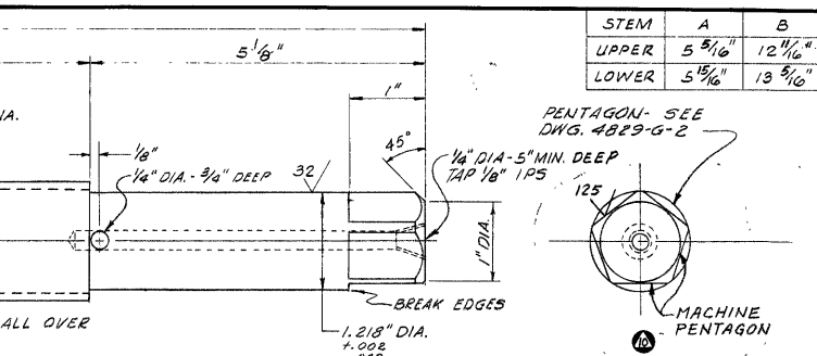
VALVE STEM
