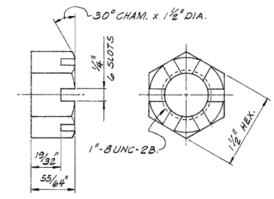
SLOTTED NUT
