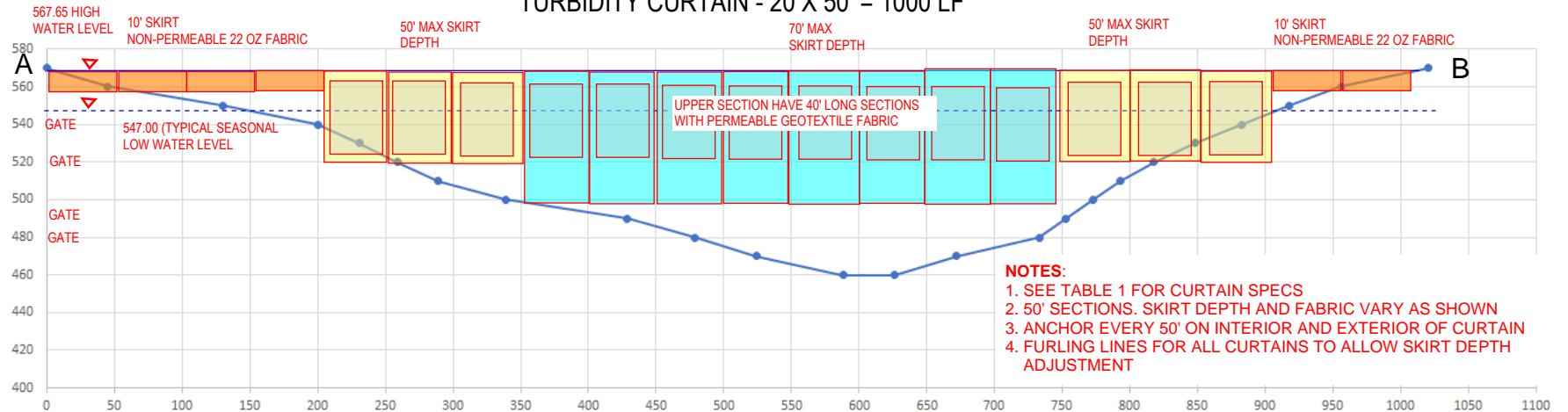
TURBIDITY CURTAIN - 20 X 50' = 1000 LF
