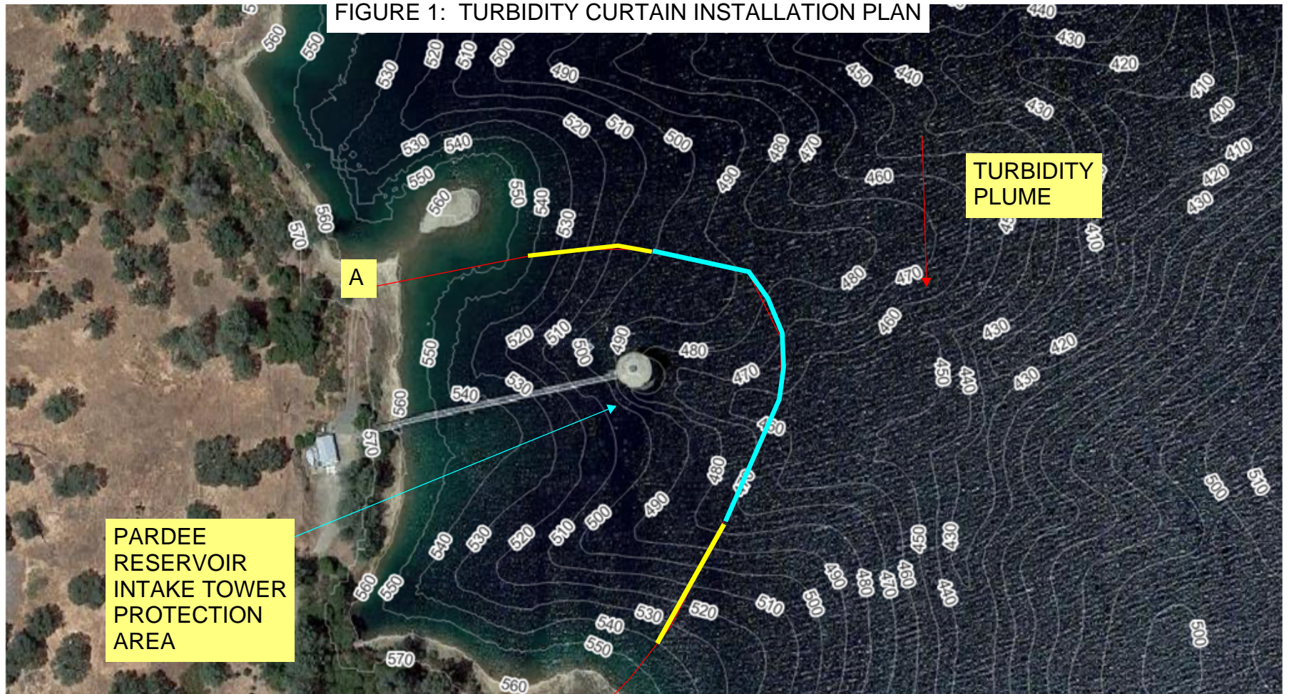
TURBIDITY CURTAIN - 20 X 50' = 1000 LF
