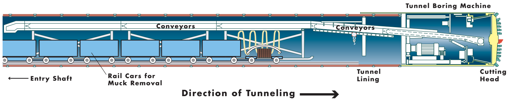
TUNNELING PROCESS
