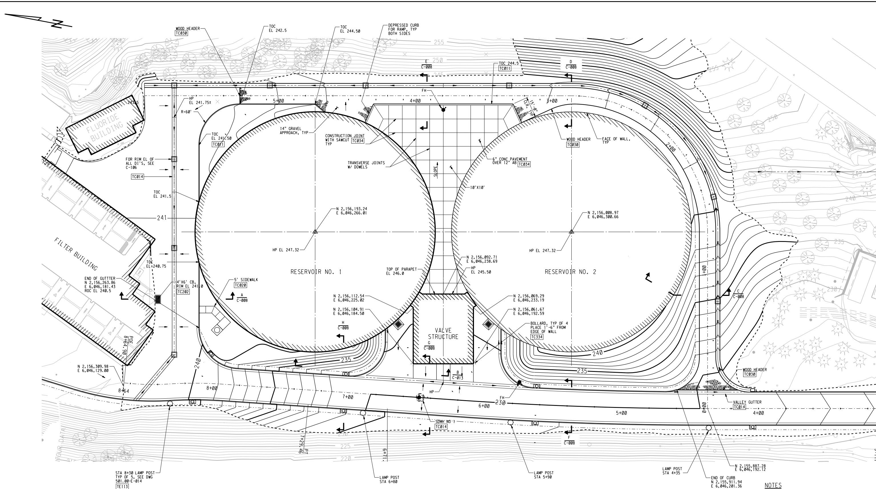
SITE PLAN 1"=20'
