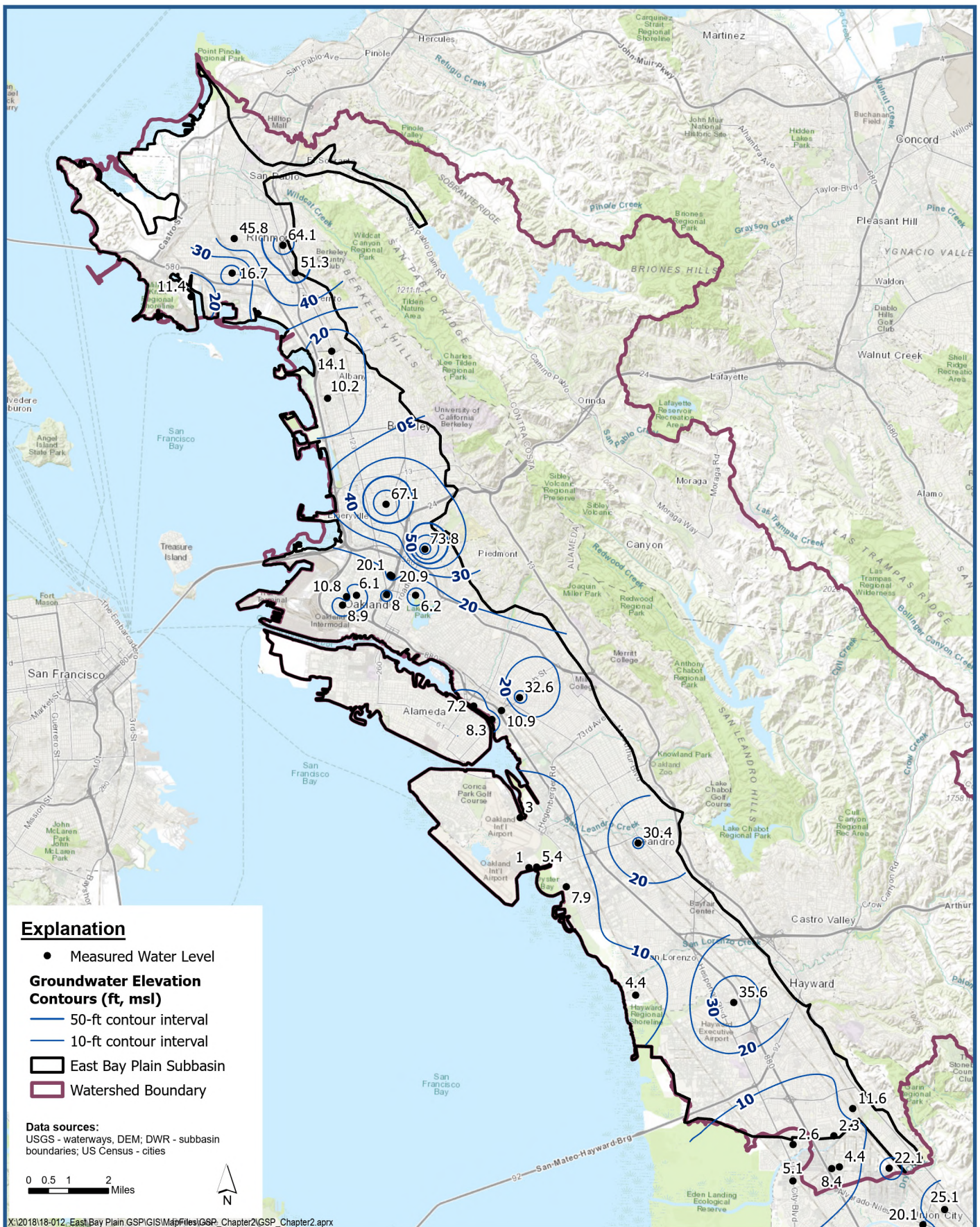
Water Table Aquifer Groundwater Elevation Contour Map – Spring 2018 East Bay Plain Subbasin Groundwater Sustainability Plan
