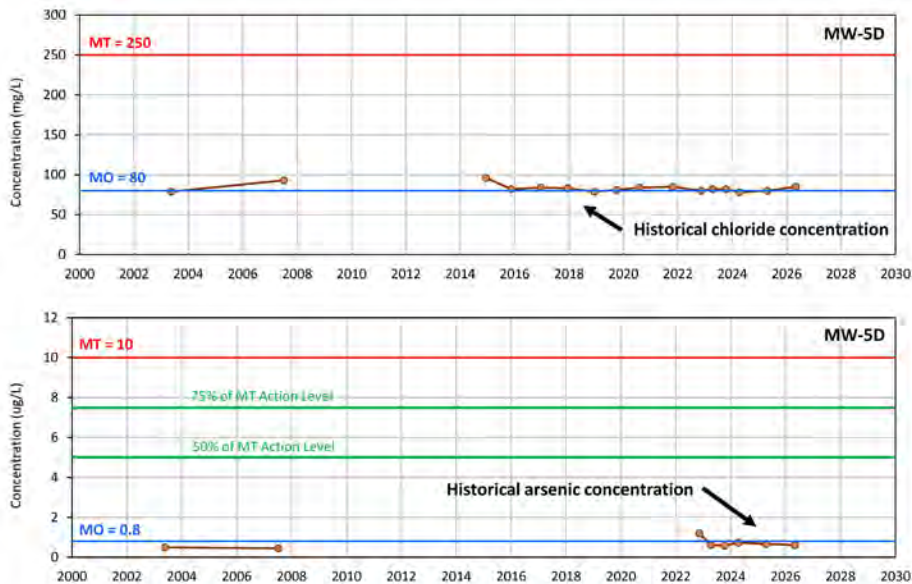
SAMPLE MONITORING WELL DATA See Appendix 3 for all locations
