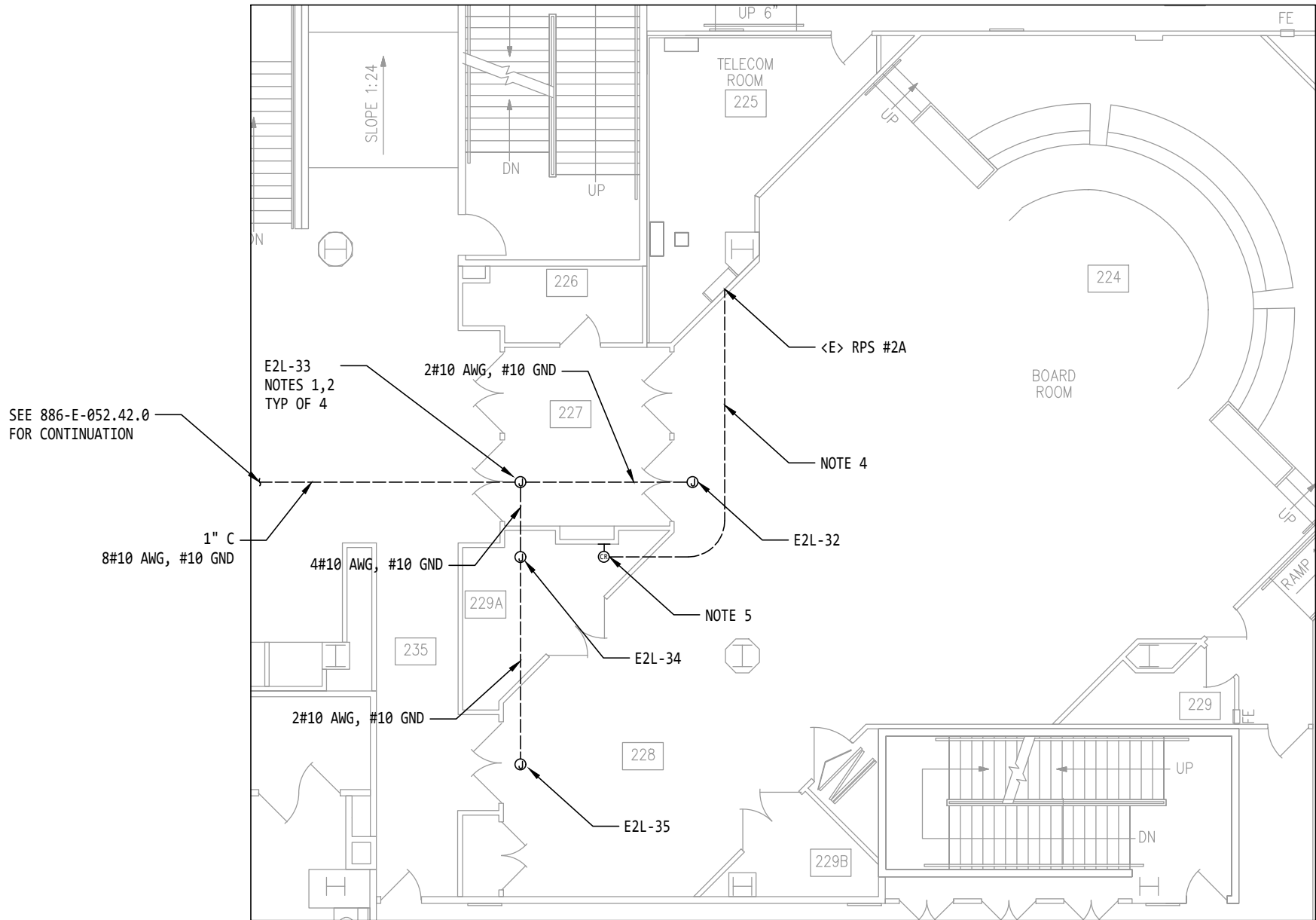
PLAN (LOCATION 3 - BOARD ROOM)
