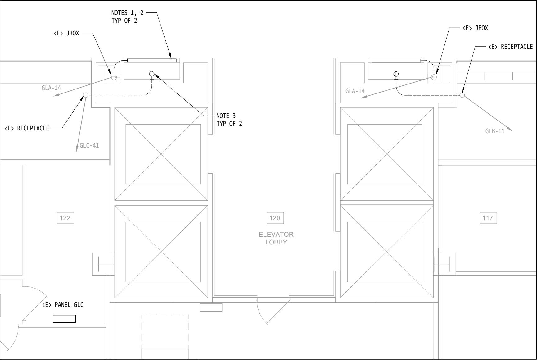
PLAN (LOCATION 1 - DISPLAY CASE) \frac{3}{8}" = 1'-0"
