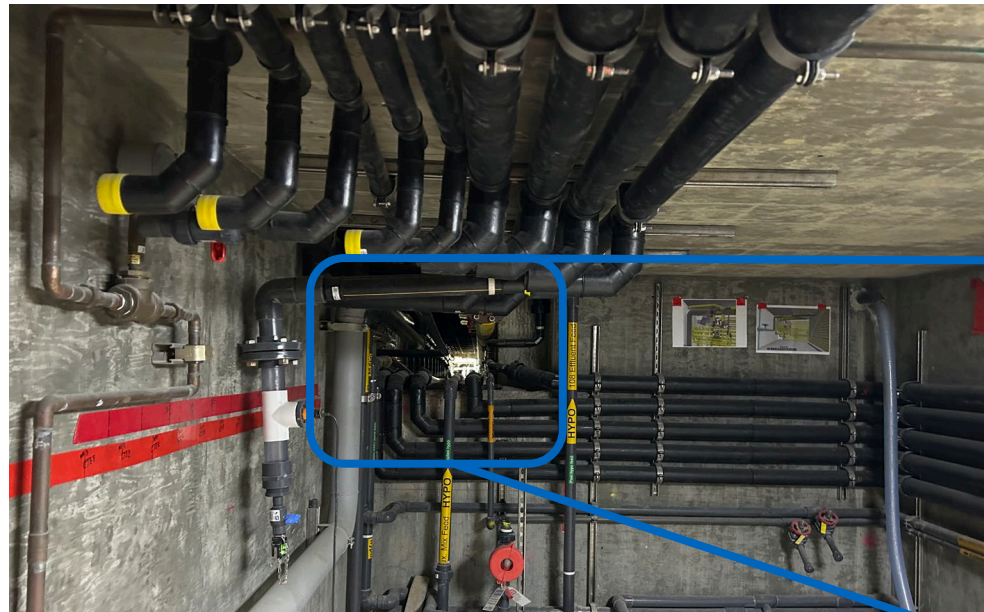
View Inside Chemical Building at Sobrante WTP, Showing Wall of Piping Entering a Chemical Trench
