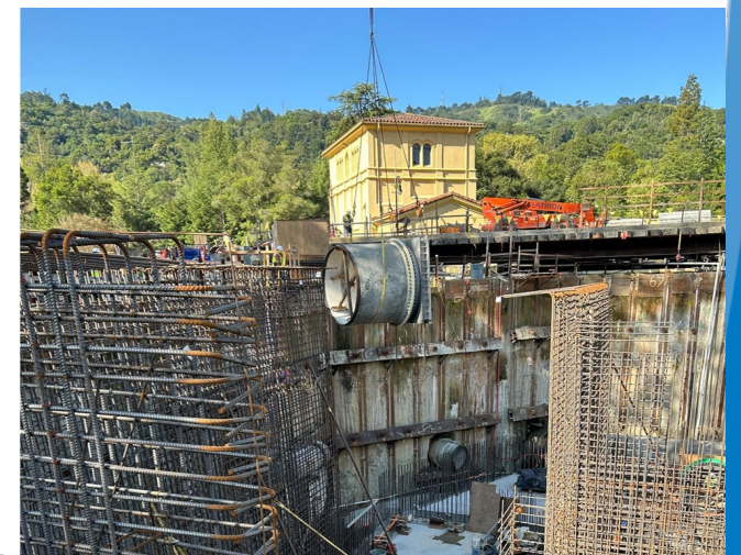
UV and CCB Structure Rebar and Piping
