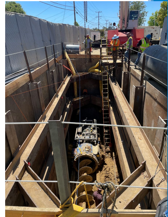
Typical Trenchless Installation
